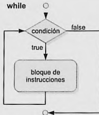
Figura 3.1. Bucle while
