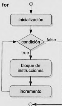
Figura 3.3. Bucle for
