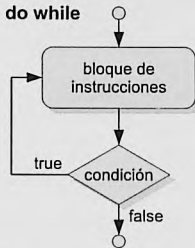
Figura 3.2. Bucle do-while
